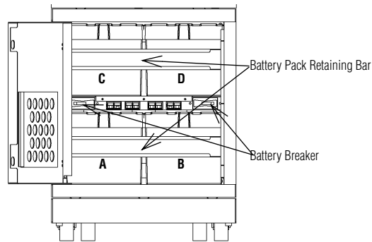
Fig. 1: ONXBC Battery Cabinet Front
